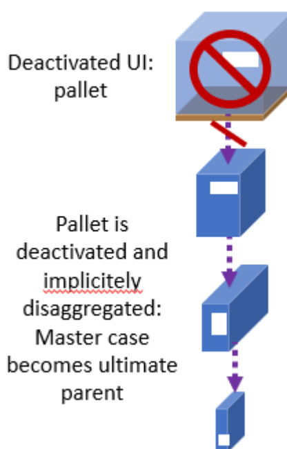
Figure 7 Implicit disaggregation triggered by a IDA Deact_Reason1 = 3,4,5 or 6
