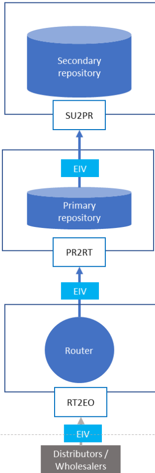
Figure 39 Data Flow Diagram – Issuing of invoice – Report from Distributors and Wholesalers
