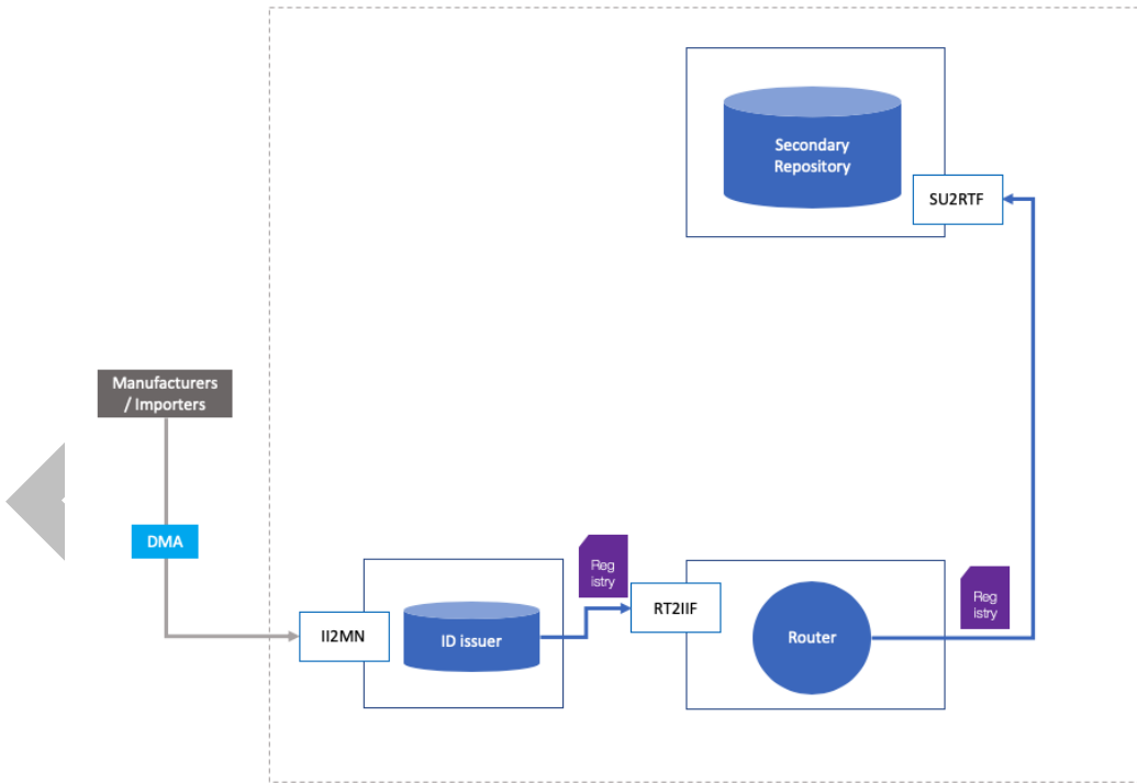
Figure 17 Data Flow Diagram – De-registration of a Machine
