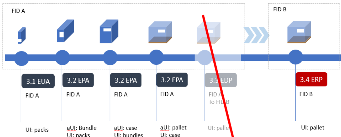
Figure 8 Arrival sequence error ARRIVAL_NOTALLOWED
