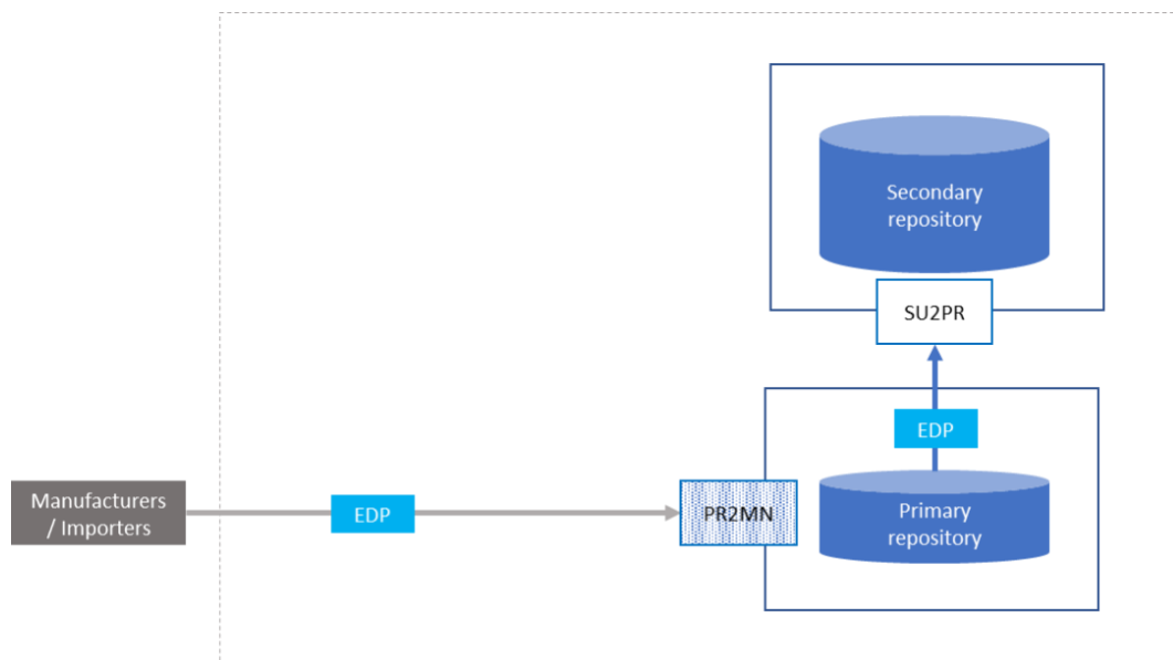
Figure 33 Data Flow Diagram – Dispatch of tobacco products from a Facility – Report from Manufacturers and Importers
