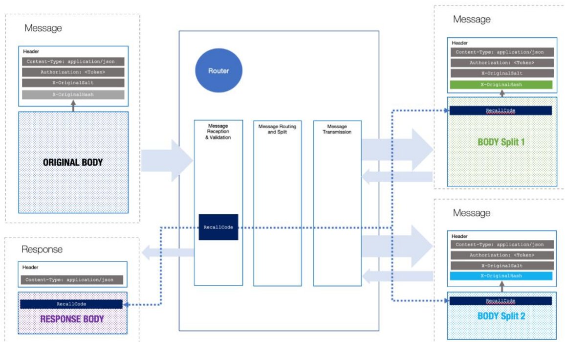
Figure 61 Recall Flow
