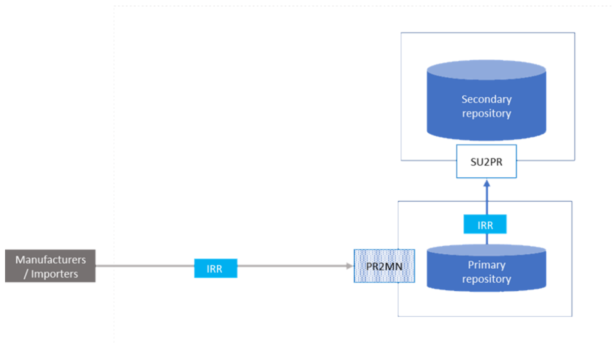
Figure 28 - Data Flow Diagram – Request for reactivation of UIs reported as stolen – Request from Manufacturers and Importers
